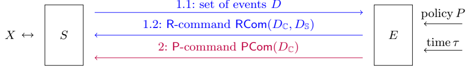
Fig. 2. System model for proactive real-time first-order enforcement
