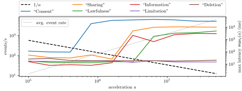
Fig. 9. RQ2: Maximum latency of WHYENF and event rate for the formulae in Figure 8.
